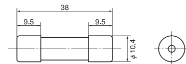
Fuse Holder HK1038 (for 660CF) refer to p. 30
