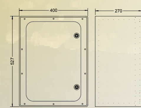
wall mounting box "Zirl" with transparent 10 mm plastic swinging door
