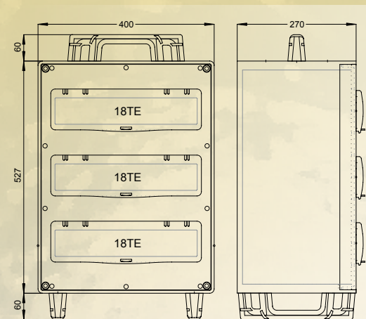
mobile solid rubber distribution box "Zirl" with closed cover
