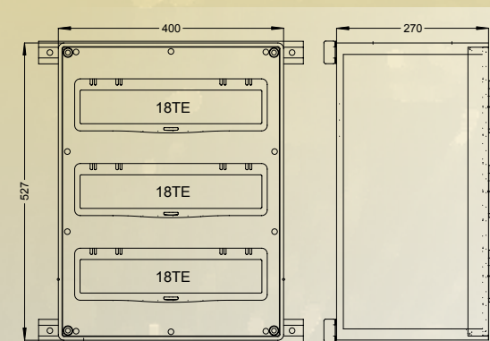
wall mounting box with window flaps
