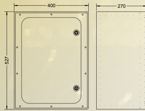
wall mounting distribution box "Zirl" with plastic swinging door
